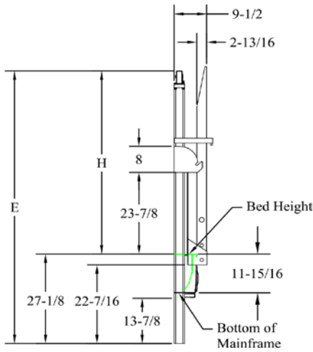
For Steel Frame / Aluminum Platform Railgates.
