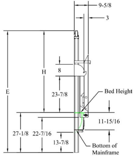
For Steel Frame / Steel Platform Railgates.
